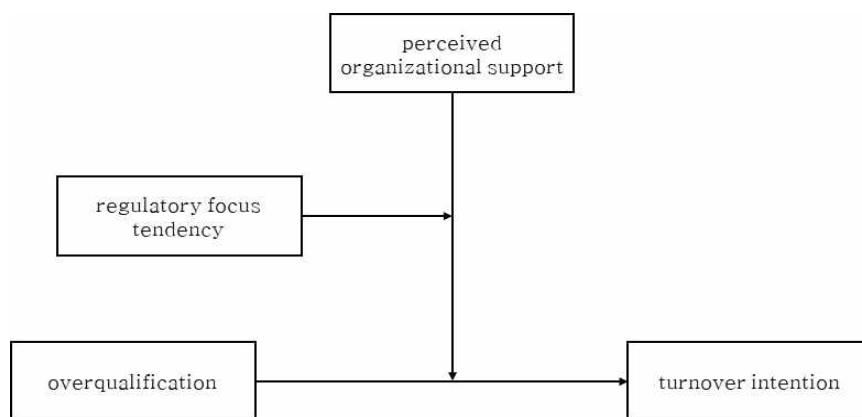
Figure 1. Hypothesis 1
