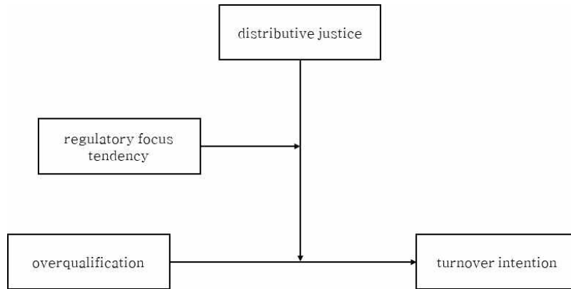
Figure 2. Hypothesis 2
