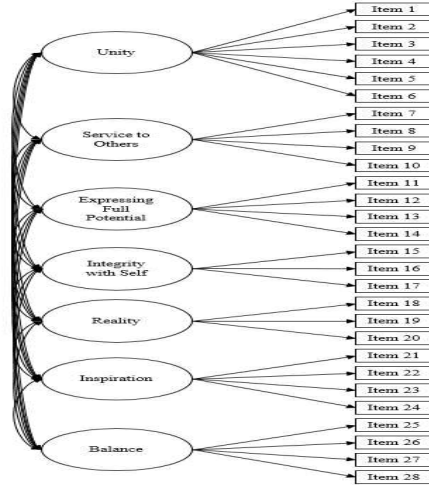
Figure 3. CFA model
