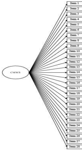
Figure 2. 1 factor model
