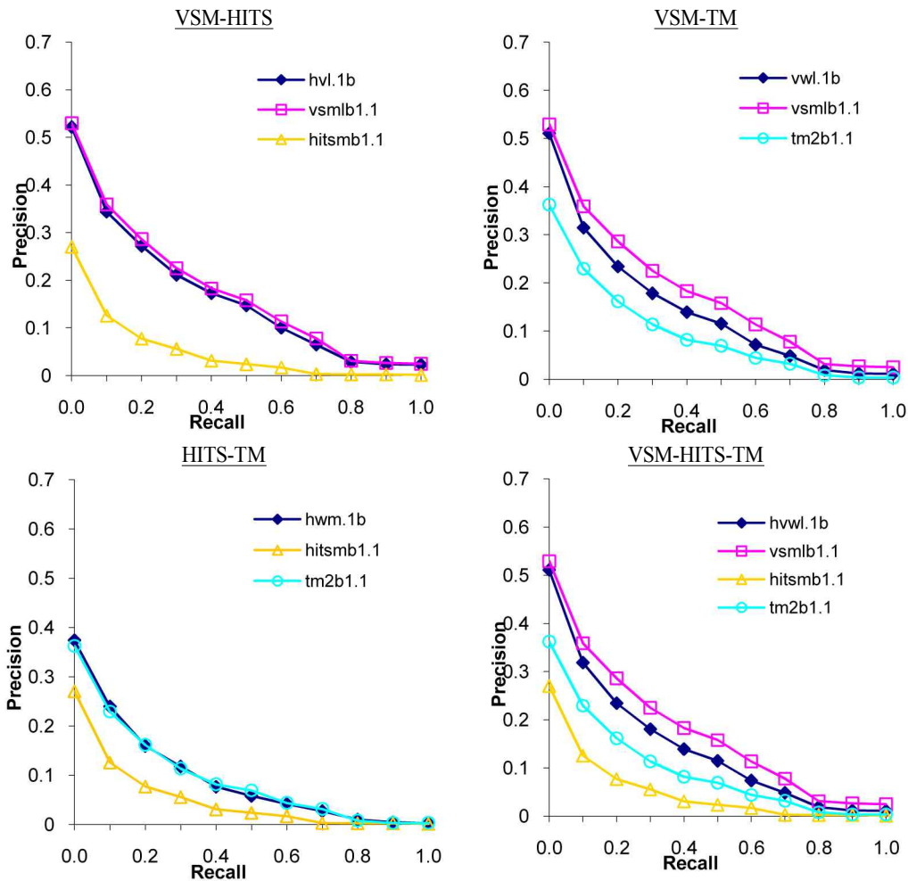
<Fig.1> Recall-Precision Curve of Inter-Fusion Systems by Method Combination
